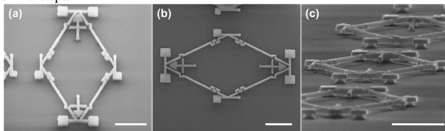
Fig. 5. SEM images of the fabricated proof-of-principle device from different perspectives. The scale bars are 3 \mu\text{m} in each image.
