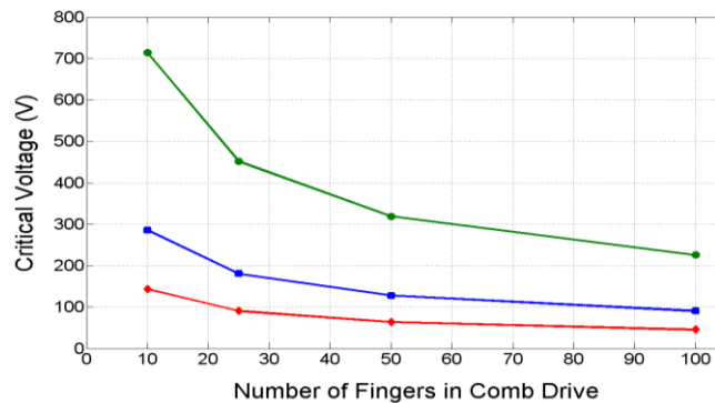
Fig. 2. Number of Fingers ( N ) vs. Critical Voltage ( V_{critical} ) for beams with different lengths. Top green curve is for 2 \mu\text{m} , blue curve is for 5 \mu\text{m} and red curve is for 10 \mu\text{m} long beams.
