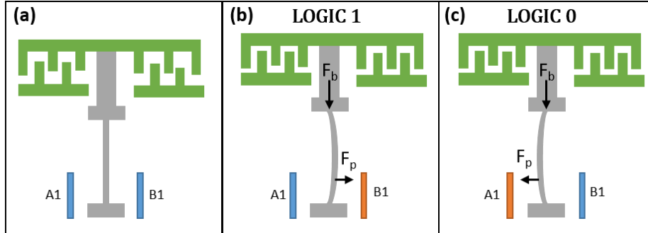
Fig. 1. Demonstration of one-bit information storage: (a) Off-state. Nanomechanical beam is shown in gray, electrodes used to preload the data are shown in blue and the comb-drive to induce buckling is shown in green (b) On-State Logic 1: A voltage is applied to B1 gate to first preload the beam (exerting F_p ), then the beam is buckled to the right by the application of buckling force F_b . (c) On-State Logic 0: A1 gate first preloads the beam, which is then buckled to the left.
